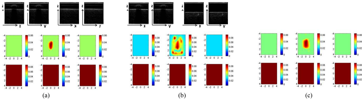
Fig. 2 Effect of depth mismatch when the two layer interface distance from the probe is deeper at the reference site compared to the target site. Top pictures in part (a) show two orthogonal ultrasound images of the target site (two left images) and reference site (two right images). Both sites have second layer located at 1.4cm depth. Target is located at x=0, y=0 and z=0.9 cm. (a) Reconstructed image of the target in case of no mismatch. Top pictures in Part (b) show two orthogonal ultrasound images of the target and reference sites when the second layer at the target and reference sites are located at 1.4cm and 2.0cm, respectively. (b) Reconstructed image of the absorption coefficient of the target before applying the mismatch correction, and (c) after applying the mismatch correction formula.
